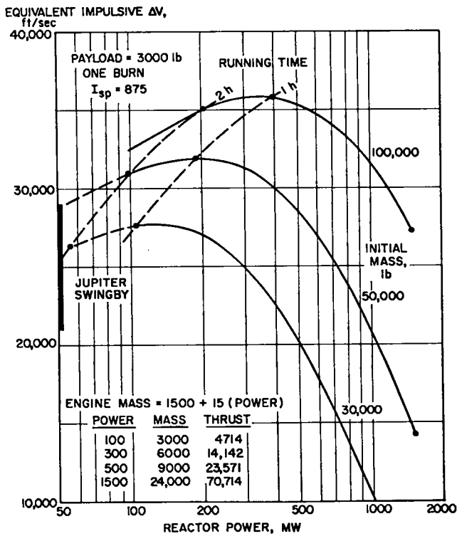
Fig. 3. Equivalent \Delta V as a function of power for a 3000-lbm payload.
