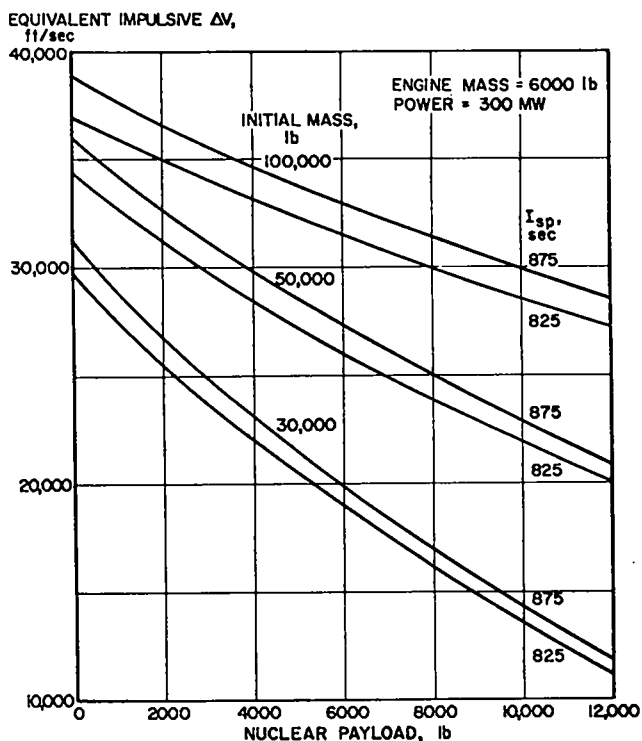
Fig. 5. Equivalent \Delta V for a 300 MW/6000 lbm engine.
