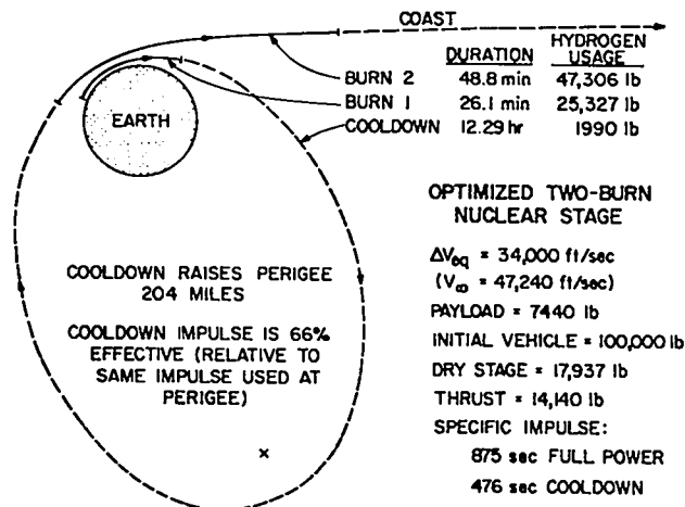
Fig. 8. Orbit schematic for a two-burn escape maneuver with cooldown considered.
