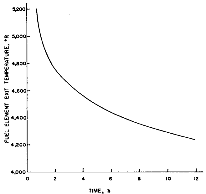
Fig. A.4. Estimated fuel-element time-versus-temperature performance.
