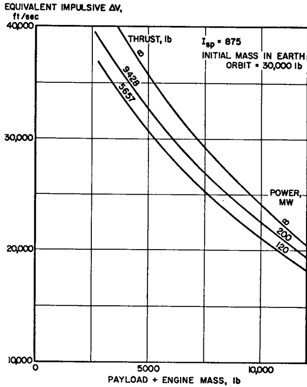
Fig. 1. Equivalent \Delta V for an initial mass of 30 000 lbm.
