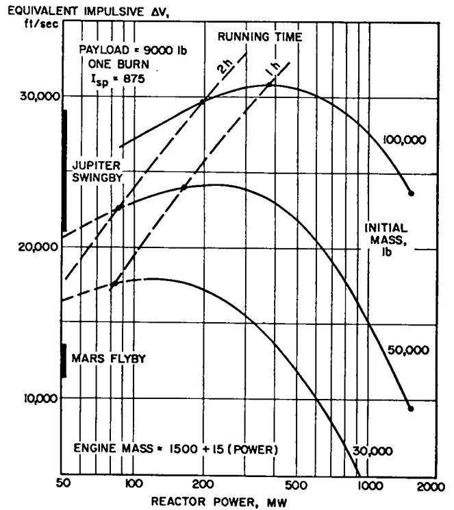
Fig. 4. Equivalent \Delta V as a function of power for a 9000-lbm payload.
