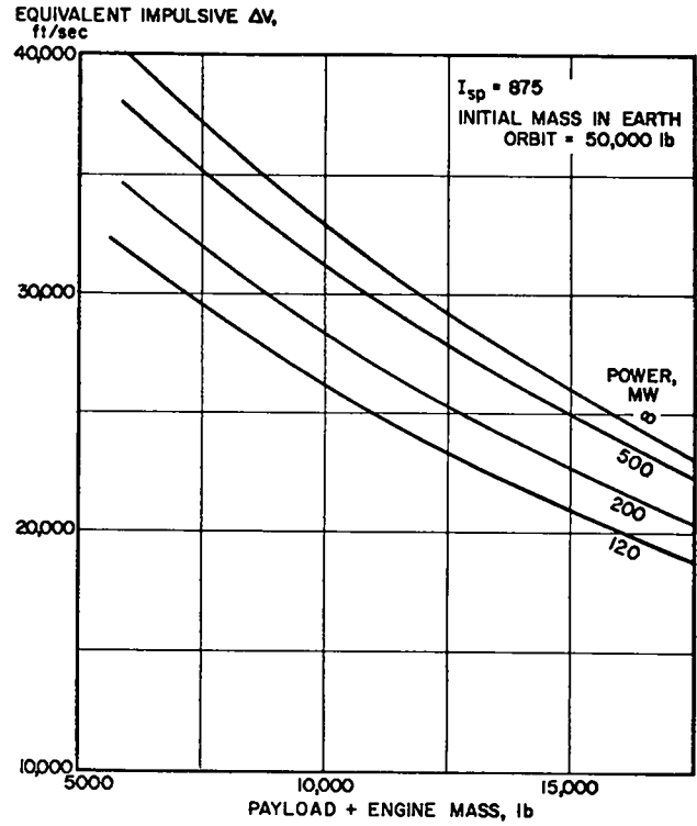
Fig. 2. Equivalent \Delta V for an initial mass of 50 000 lbm.
