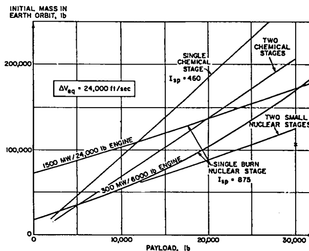
Fig. 6. Vehicle mass requirements for a 24 000 ft/sec mission.
