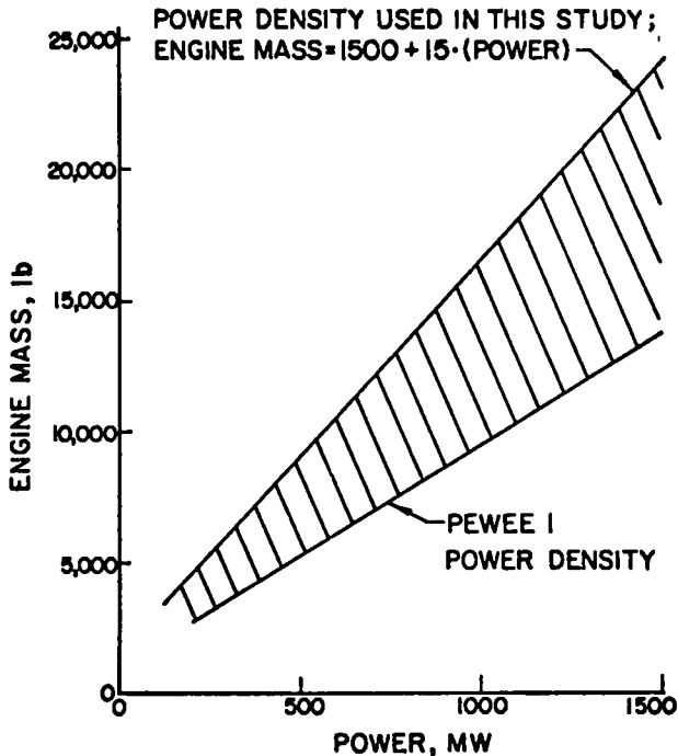
Fig. A.3. Estimated engine mass versus power.
