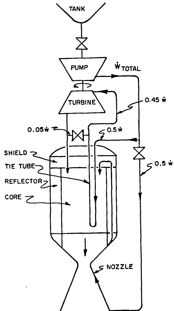
Fig. A.1. Engine cycle schematic.
