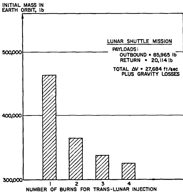
Fig. 11. Initial mass requirements for a lunar shuttle vehicle using a small nuclear engine.
