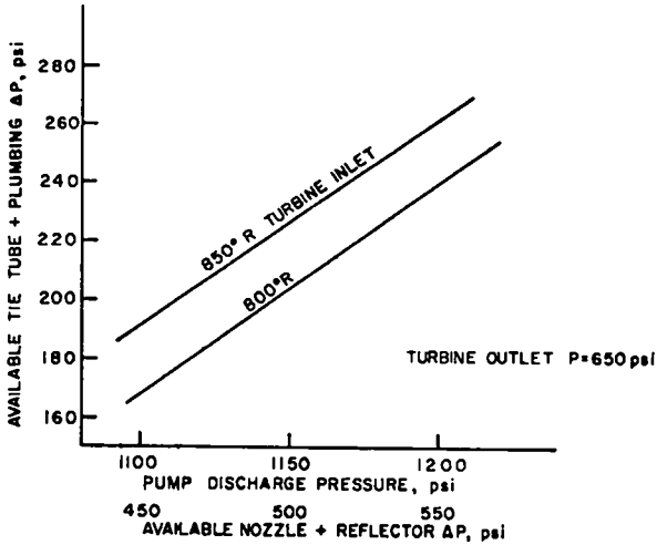
Fig. A.2. System pressures and pressure drops.
