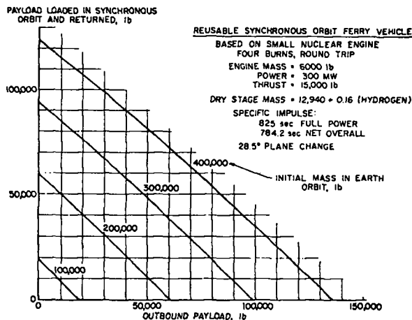
Fig. 12. Initial mass requirements for a synchronous orbit ferry vehicle.
