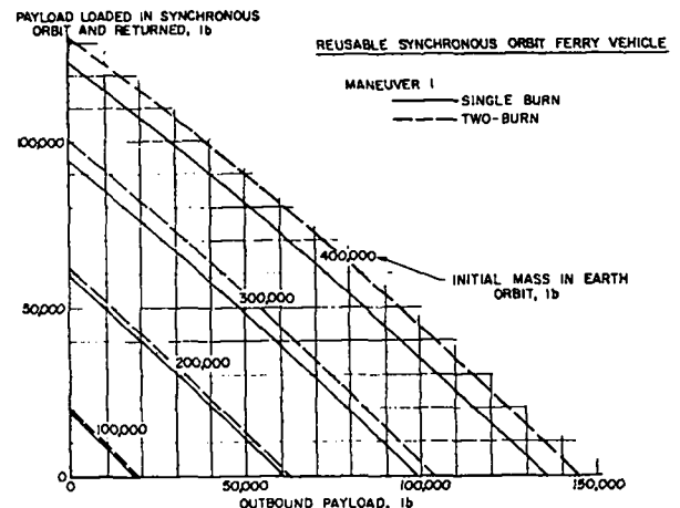
Fig. 13. Effect of two-burns for Maneuver 1.
