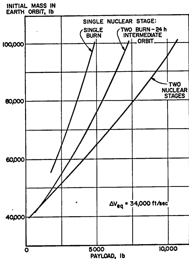
Fig. 7. Vehicle requirements for a 34 000 ft/sec mission.
